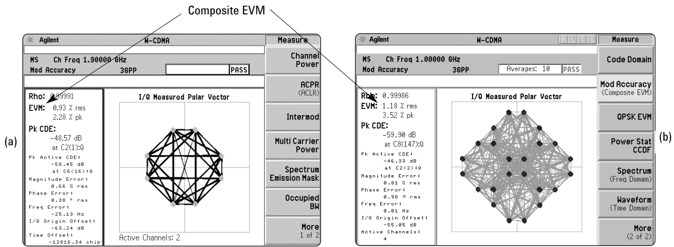
Figure 20. Composite EVM and vector diagram for a signal with (a) UL 12.2 kbps reference measurement channel (one DPDCH and a DPCCH), and (b) three DPDCHs and a DPCCH.
