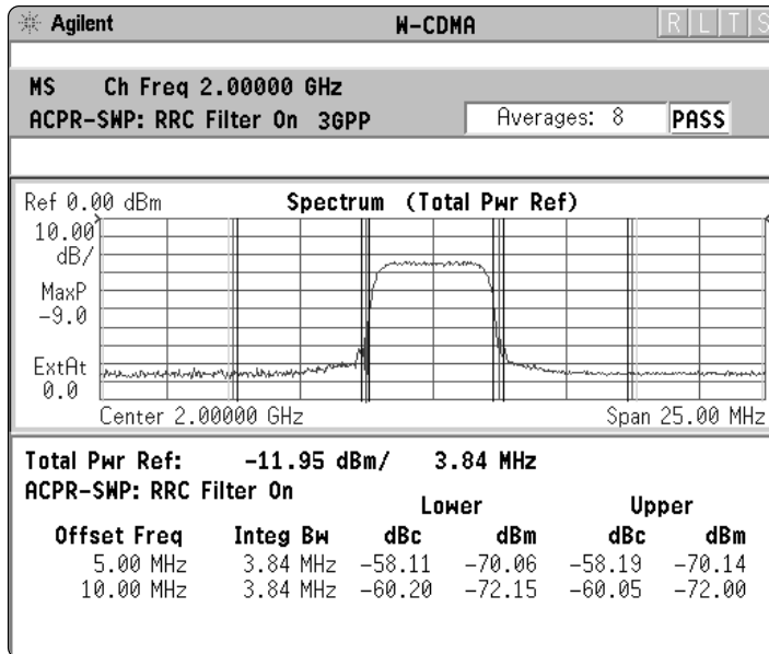
Figure 12. ACLR measurement for W-CDMA UE transmitter using a RRC filter as specified [12]
