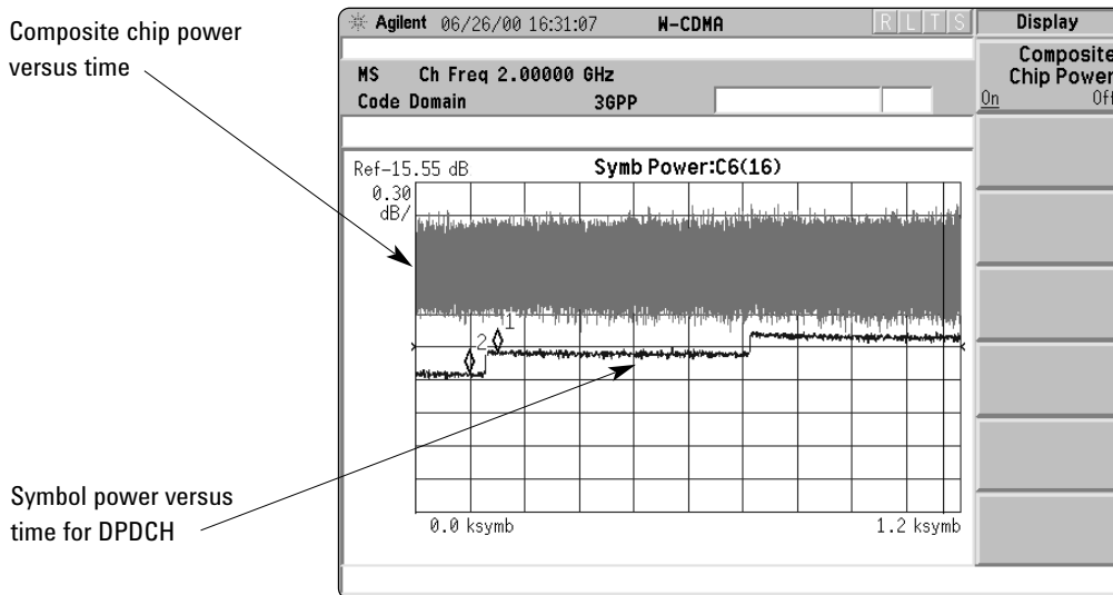
Figure 30. Chip power versus time for a W-CDMA UL signal with the DPCCH and one DPDCH at 60 kbps ( C_{ch,64,16} ), combined with symbol power versus time for the DPDCH ( C_{ch,64,16} ).
