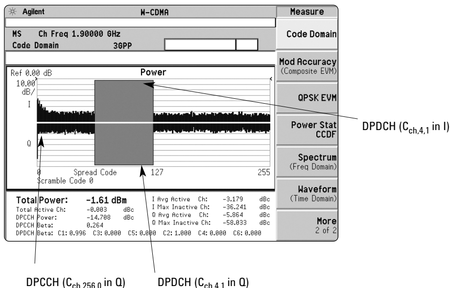
Figure 25. Code domain power measurement for the UL 768 kbps reference measurement model (one DPCCH and two DPDCHs). Signal with high LO instability.
