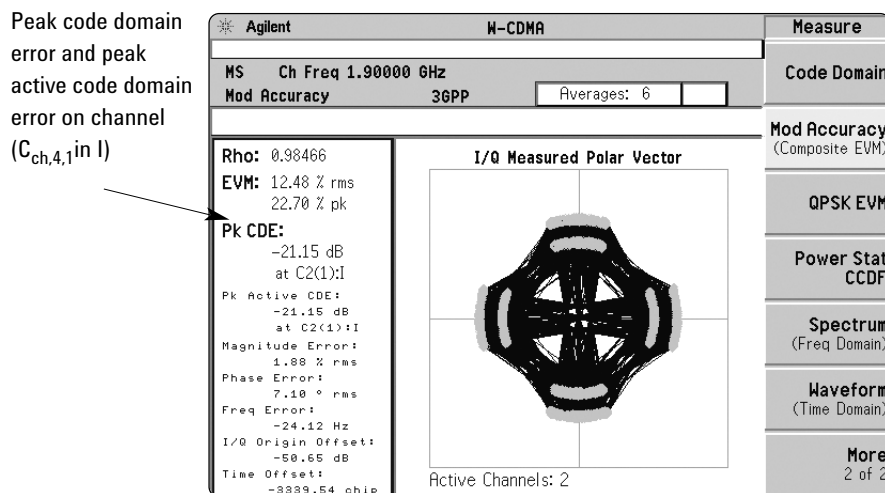
Figure 26. Peak code domain error and composite EVM display for the UL 768 kbps reference measurement model (one DPCCH and two DPDCHs). Signal with high LO instability.
