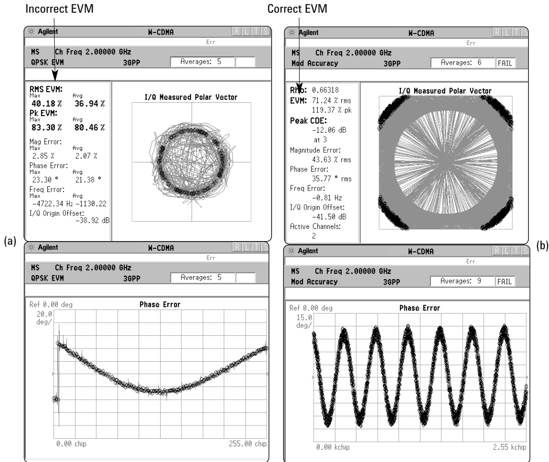
Figure 21. W-CDMA UL signal with one DPDCH and a DPCCH at the same amplitude. Signal with very high LO instability. (a) Vector diagram and phase error versus time for a QPSK EVM measurement. (b) Vector diagram and phase error versus time for a composite EVM measurement.
