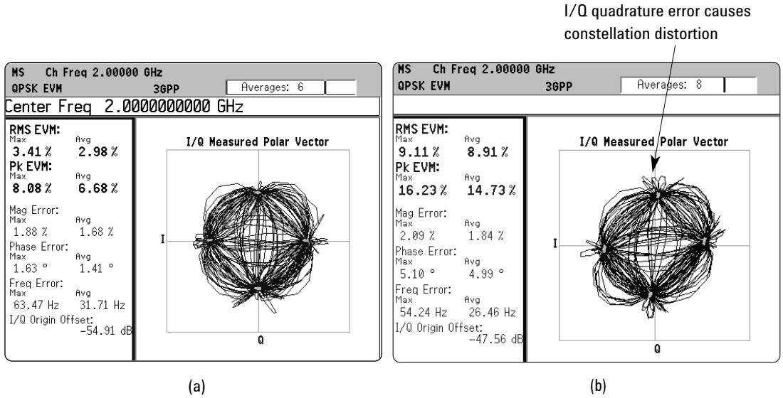
Figure 18. Vector diagram and QPSK EVM measurement for an UL W-CDMA signal (one DPDCH and one DPCCH at the same amplitude level). (a) Transmitter without any impairment. (b) Transmitter with an I/Q quadrature error.
