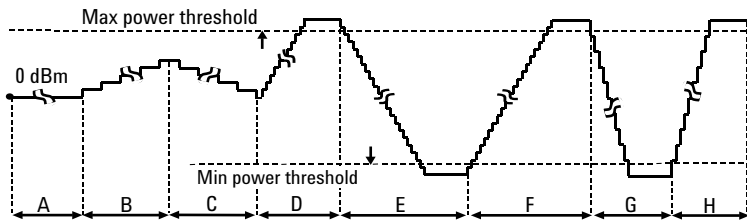
Figure 37. Pattern of power control steps defined in the inner loop power control (UL) in the 3GPP specifications [12]
